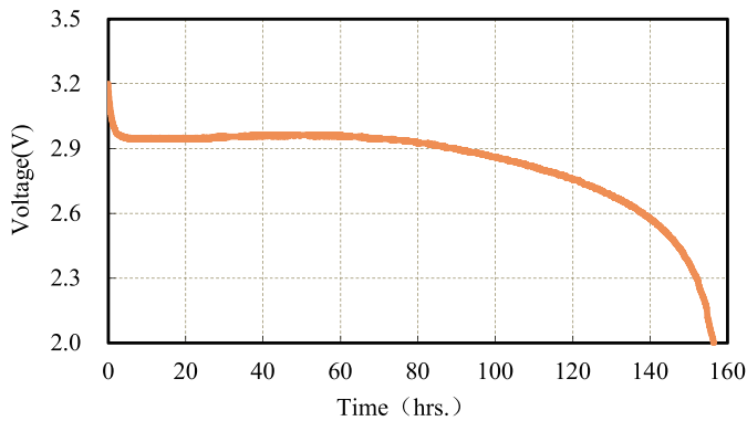
10mA continuous discharge to 2.0V at 73.4°F (23°C)
