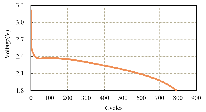
1,800mA (3s on/7s off) at 73.4°F (23°C)
