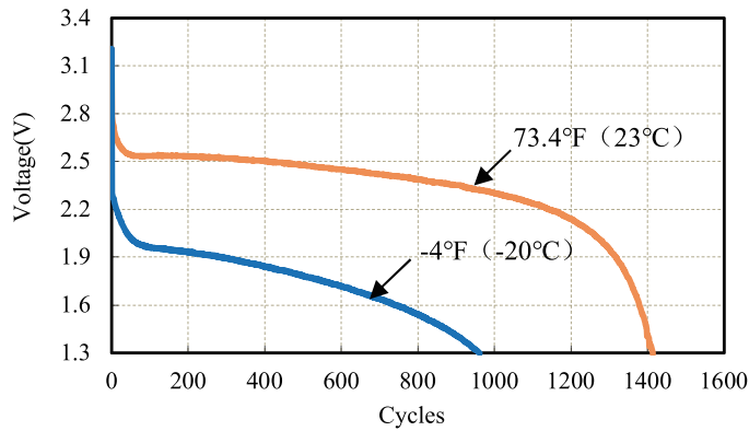
1,200mA (3s on/7s off) at 73.4°F & -4°F (23°C & -20°C)
