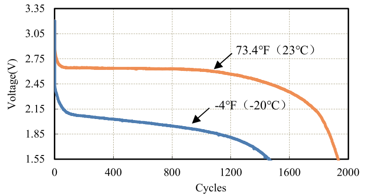
900mA (3s on/27s off) at 73.4°F & -4°F (23°C & -20°C)
